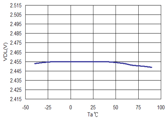
(3) V_{DL} vs. T_a
