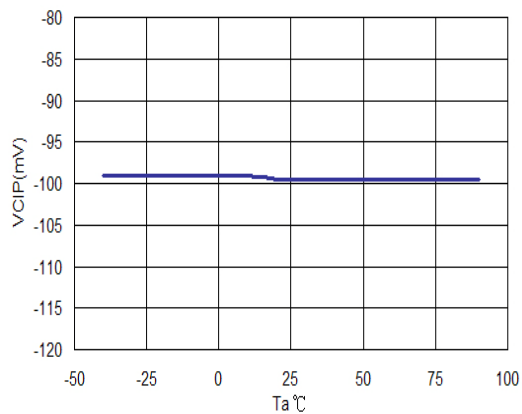
(11) V_{CIP} vs. T_a
