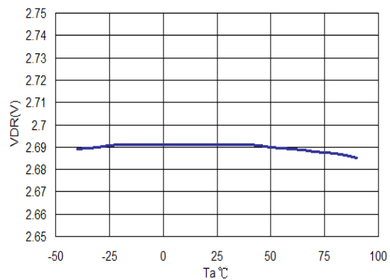
(4) V_{DR} vs. T_a
