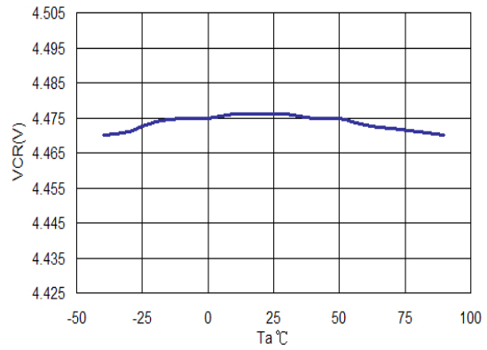
(2) V_{CR} vs. T_a
