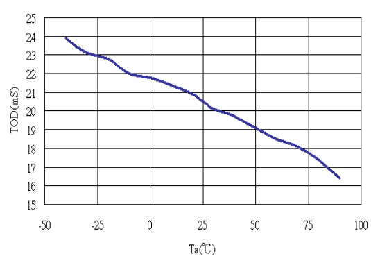
(6) T_{OD} vs. T_a
