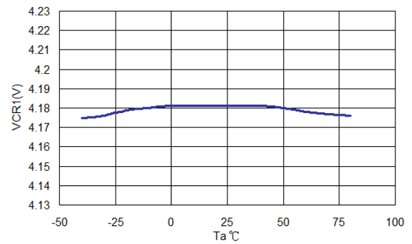
(2) V_{CR1} vs. T_a
