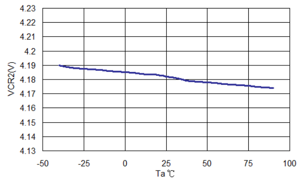
(6) V_{CR2} vs. T_a
