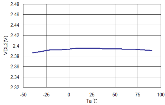
(7) V_{DL2} vs. T_a
