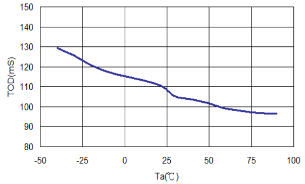
(10) T_{OD} vs. T_a
