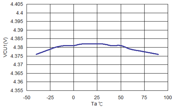
(1) V_{CU1} vs. T_a
