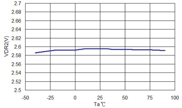
(8) V_{DR2} vs. T_a
