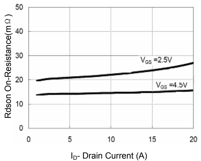
Figure 6 Drain-Source On-Resistance
